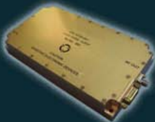
SSPA 0.020-1.000-25 20 MHz - 1000 MHz 25 Watt RF Amplifier
