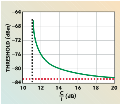
▲ Fig. 3 Threshold degradation for BER=10^{-6} .
