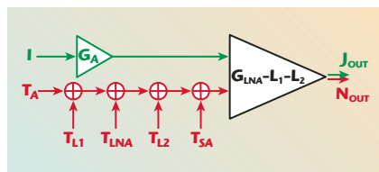
Fig. 6 System noise sources.
