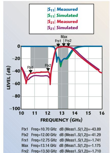
▲ Fig. 15 Electromagnetic simulated and measured responses of the modified fourth-order Ku-band DBR filter.
